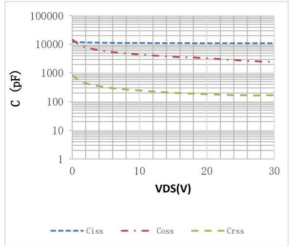
Fig.2 Capacitance Characteristics
